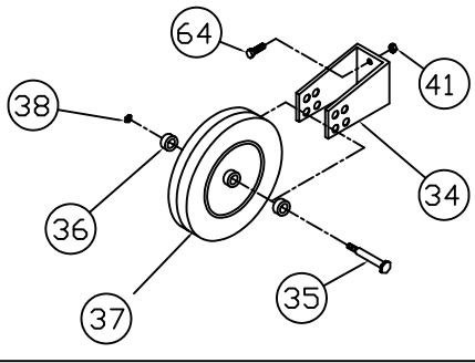
FRONT WHEEL, BRACKET AND HARDWARE LB5 LB8
